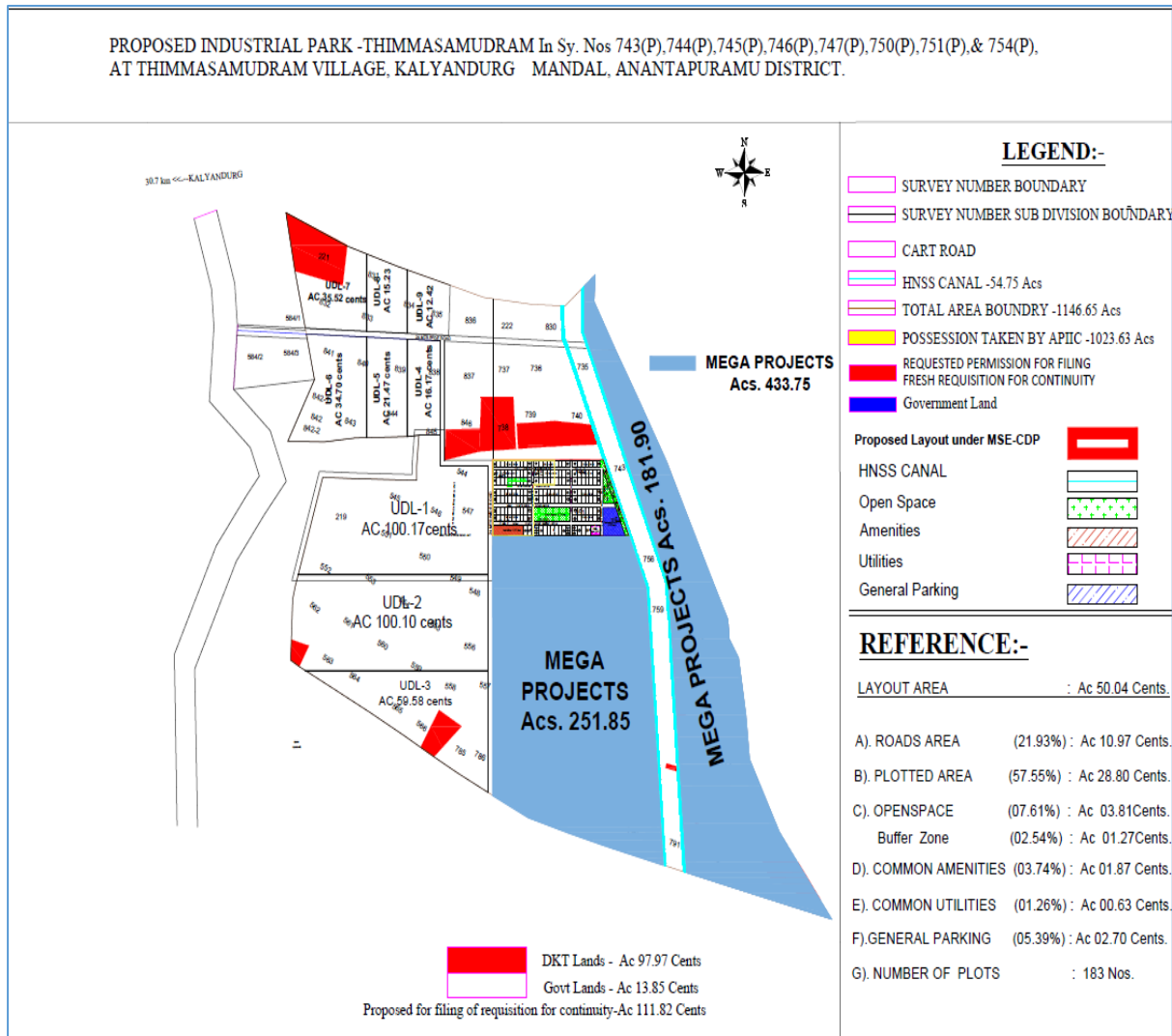
Figure 1 - Site Layout
