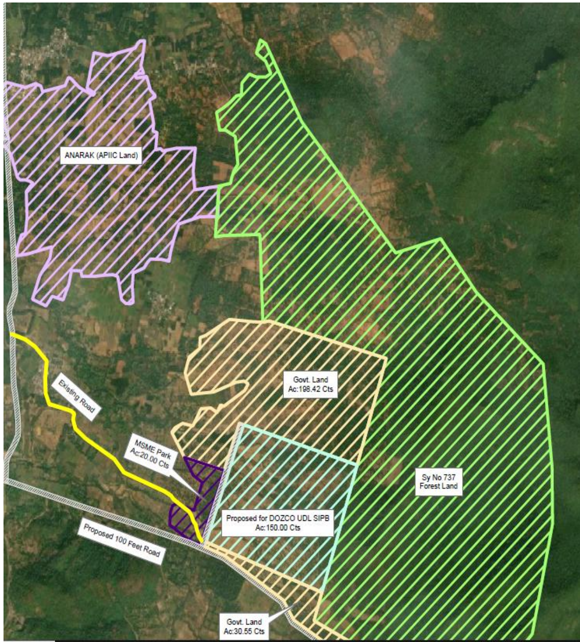
Figure 1 - Site Layout
