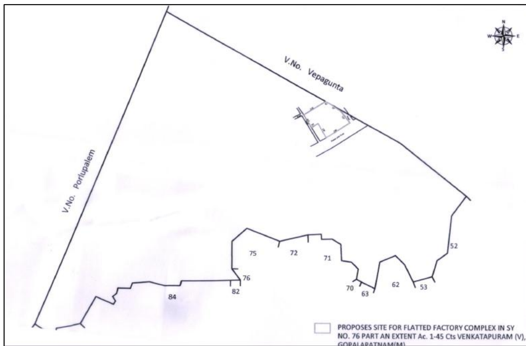
Figure 1 - Site Layout
