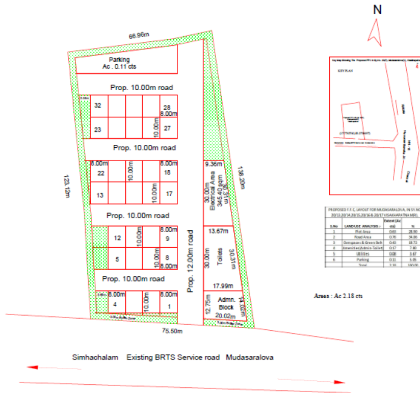
Figure 1 - Site Layout
