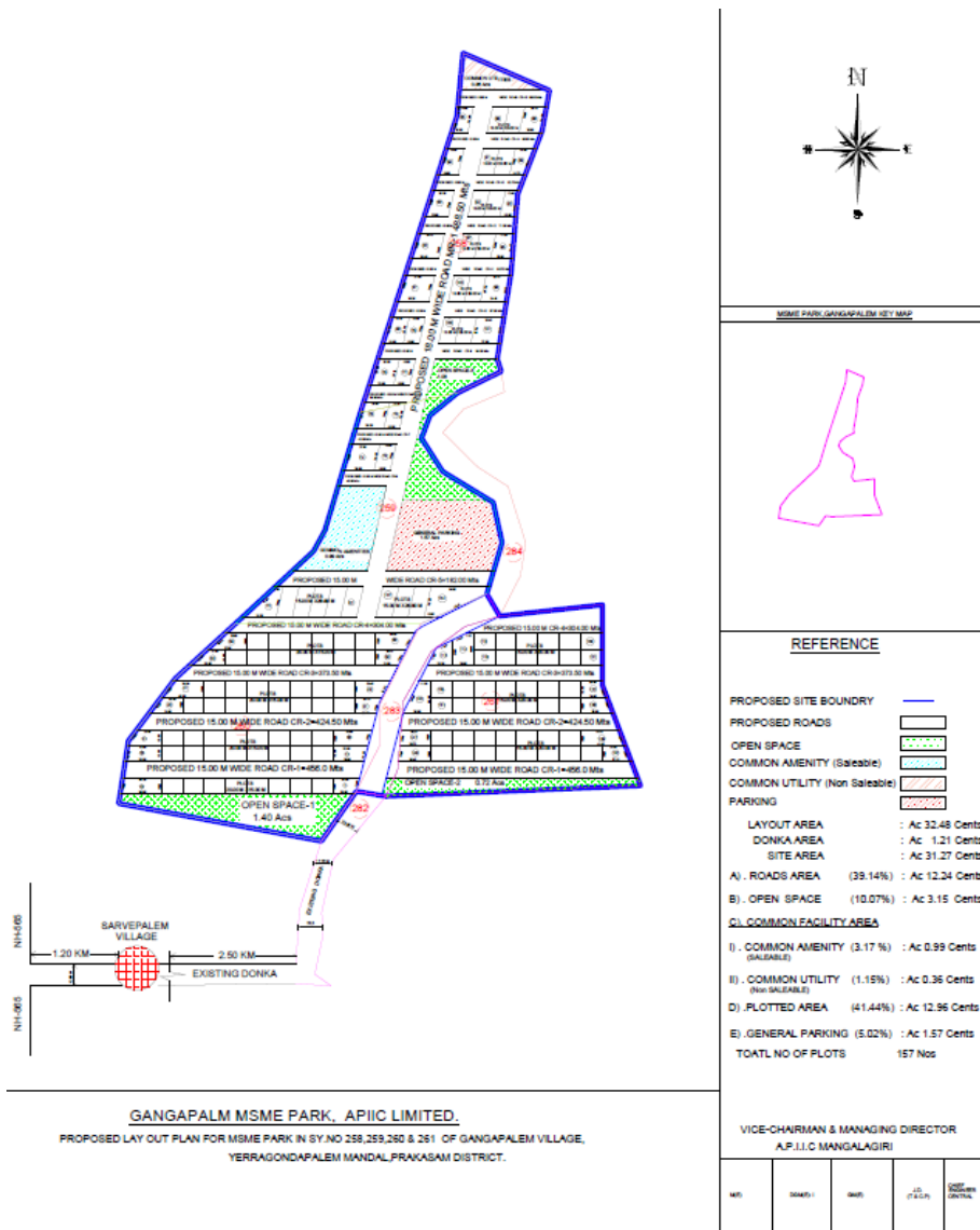
Figure 1 - Site Layout
