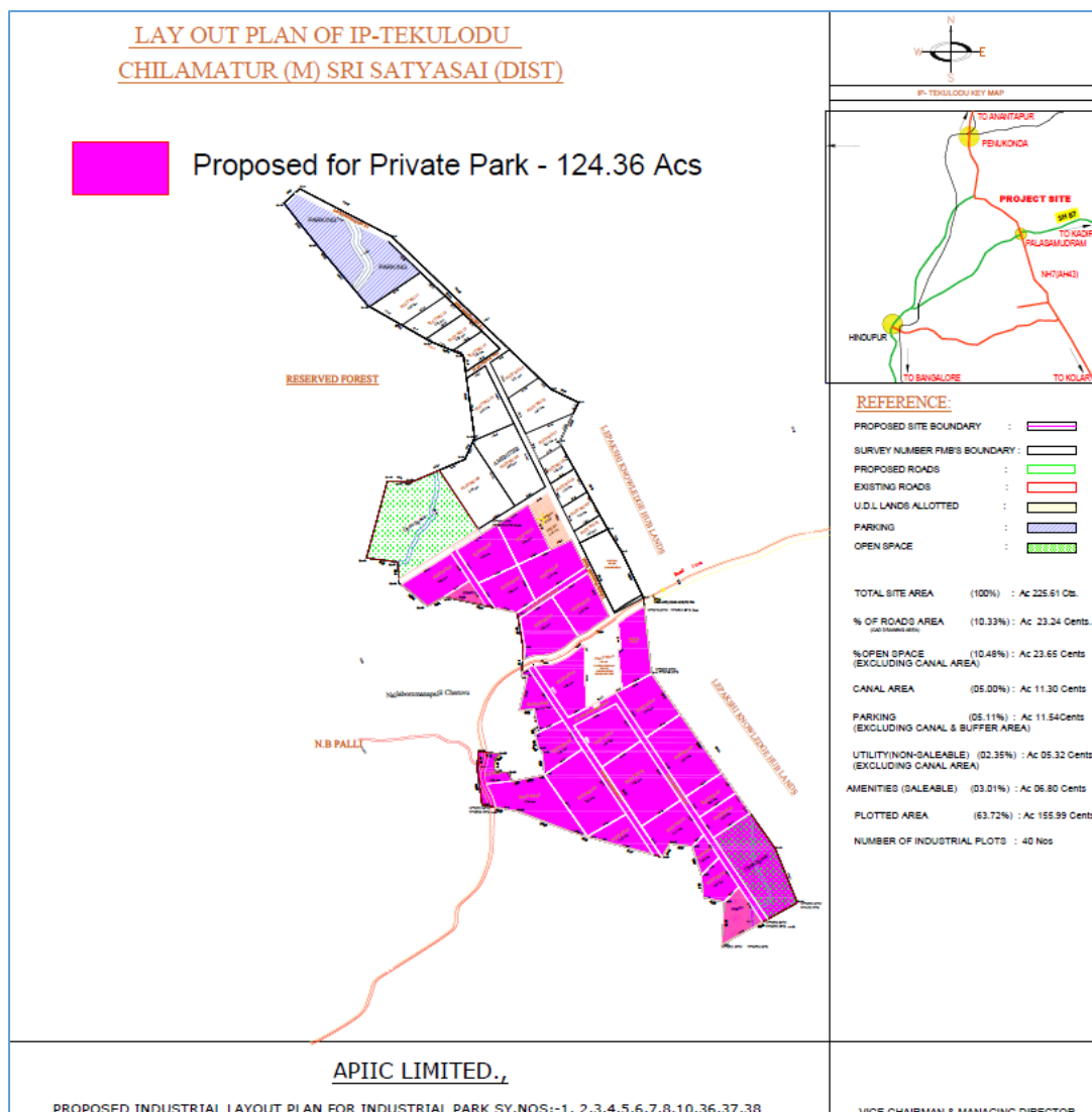
Figure 1 - Site Layout
