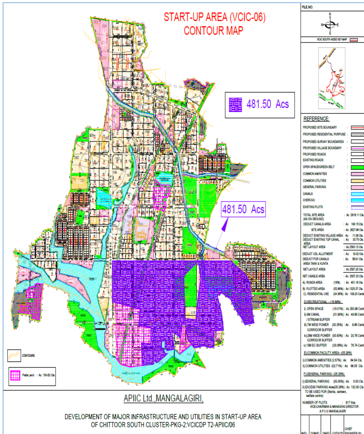
Figure 1 - Site Layout
