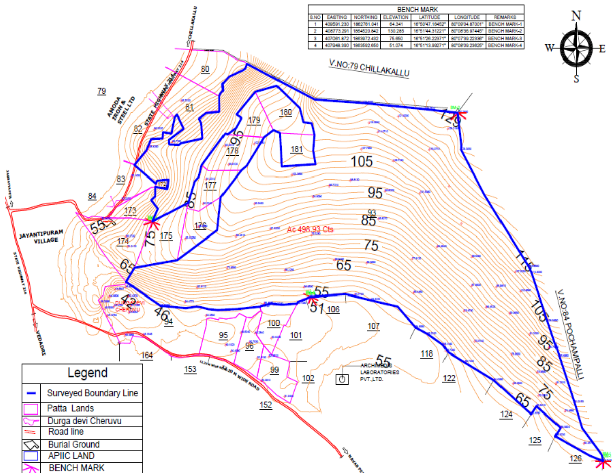
Figure 1 - Site Layout
